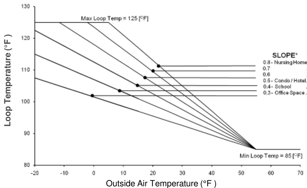
Hybrid Heat Pump Loop Temperature (°F) vs. Outside Air Temperature (°F)
