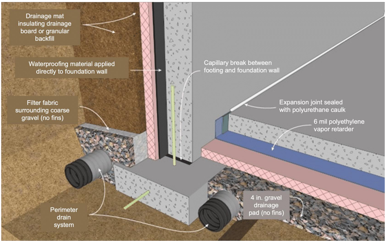
Recommended design detail DOE Foundation Design Handbook
